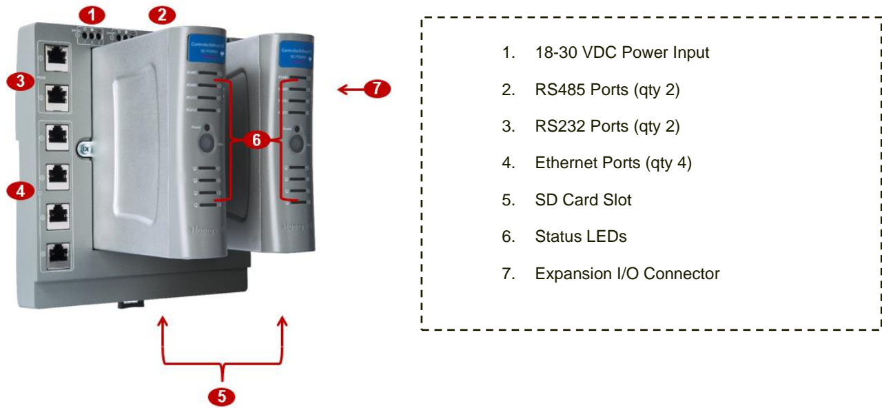
Figure 3 –Redundant Controller Hardware Summary
